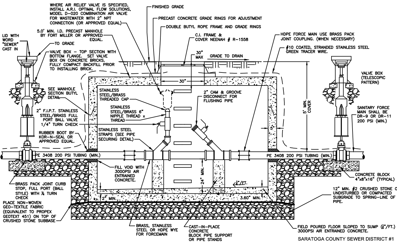
PRESSURE SANITARY SEWER IN-LINE CLEAN OUT AND AIR RELIEF STATION (OPTION 3)
